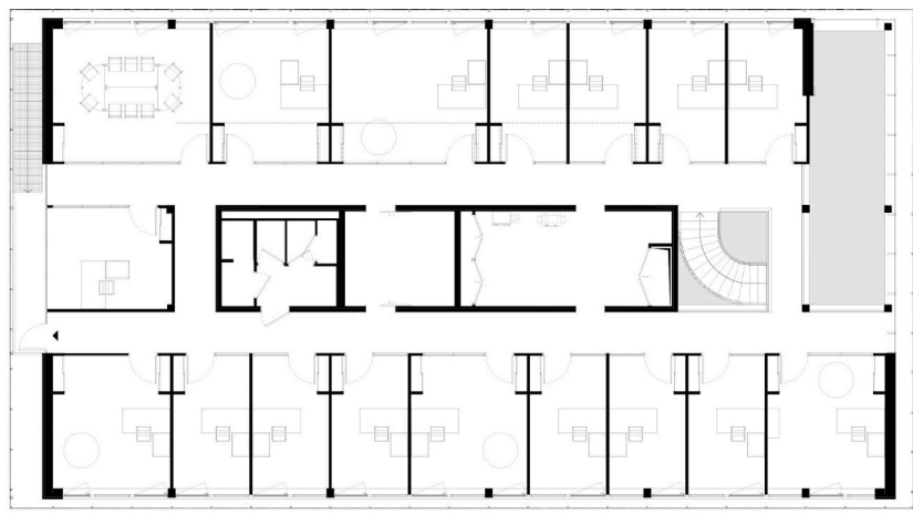
Plan R+1
